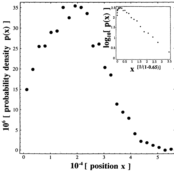
FIG. 4. Probability density p(x, t = 10^7) vs position x (total of 3000 molecules). The probability p(x, t) is in arbitrary units. The inset shows \log_{10}[p(x, t = 10^7)] vs x^{[1/(1-0.65)]} , where both expressions are in arbitrary units. See Fig. 1 for other details.
